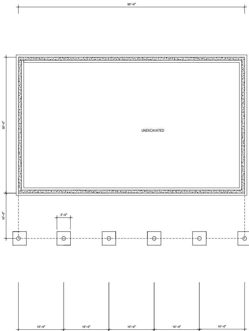
1 FOUNDATION PLAN SCALE 1/4"=1'-0"
