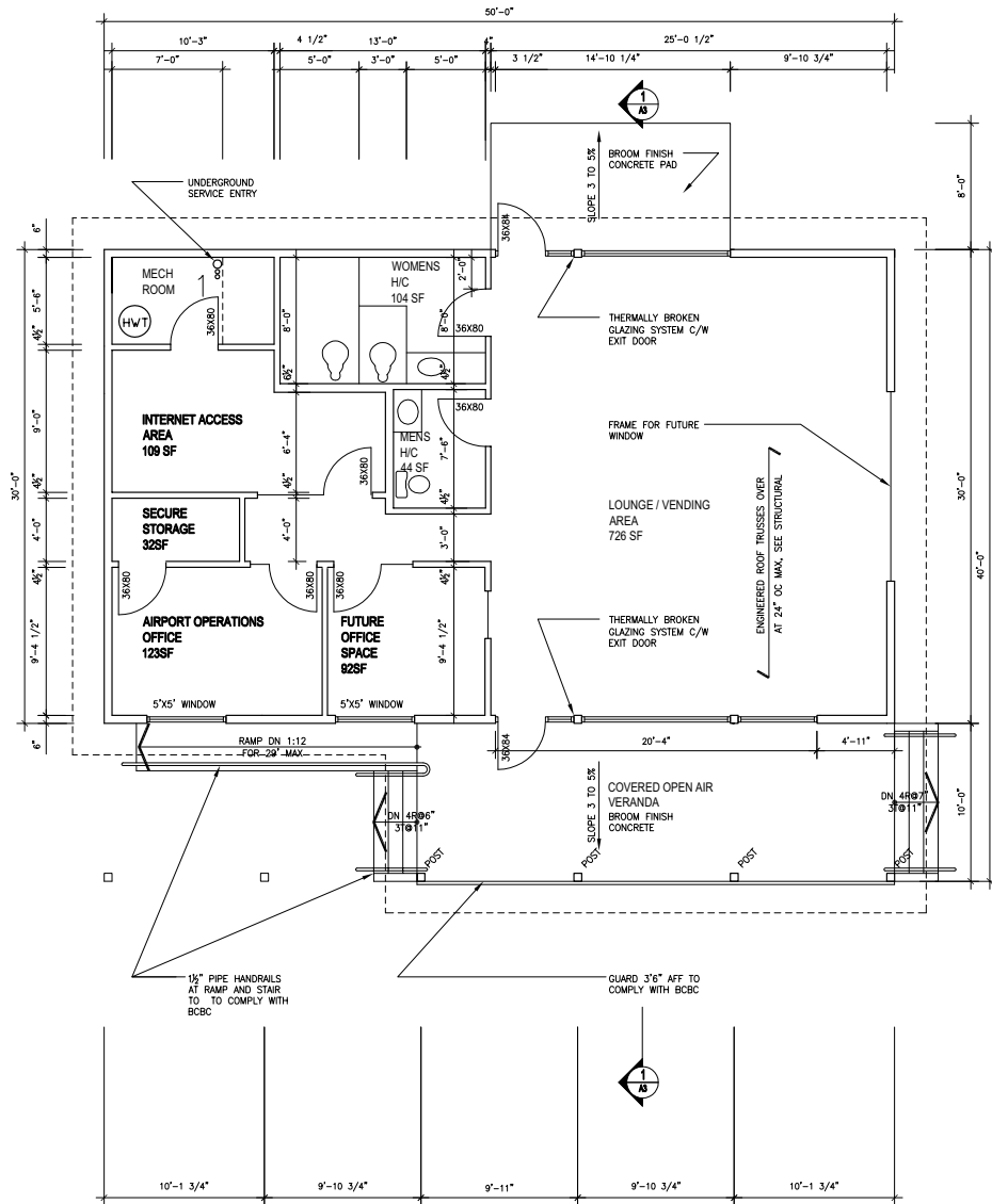
2 FLOOR PLAN SCALE 1/4"=1'-0"
